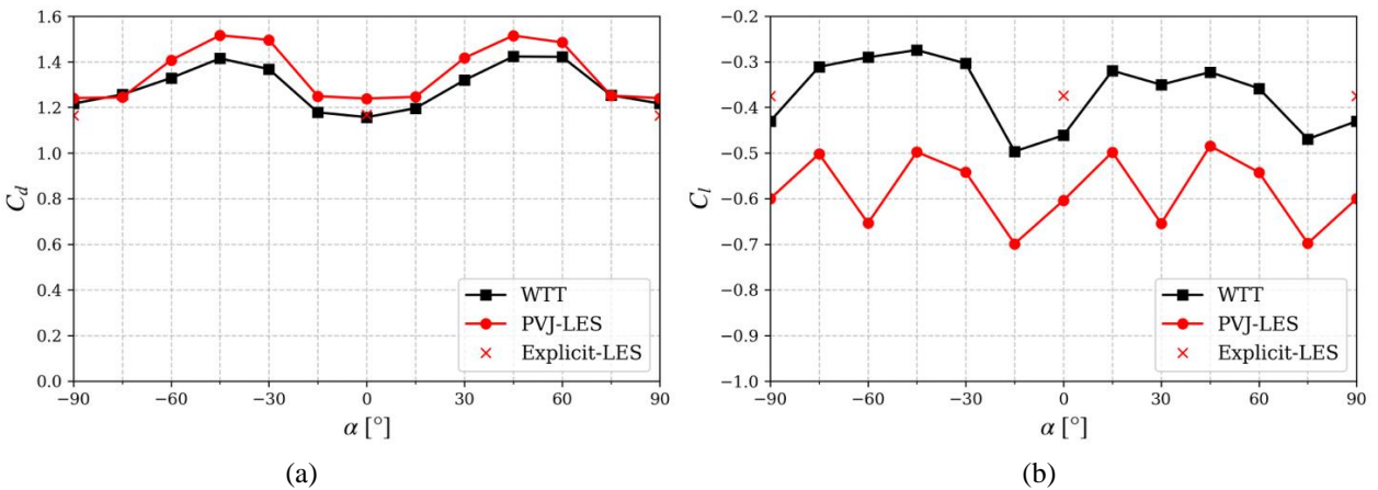
Figure 2: Force coefficients comparison: (a) drag force and (b) lift force.
