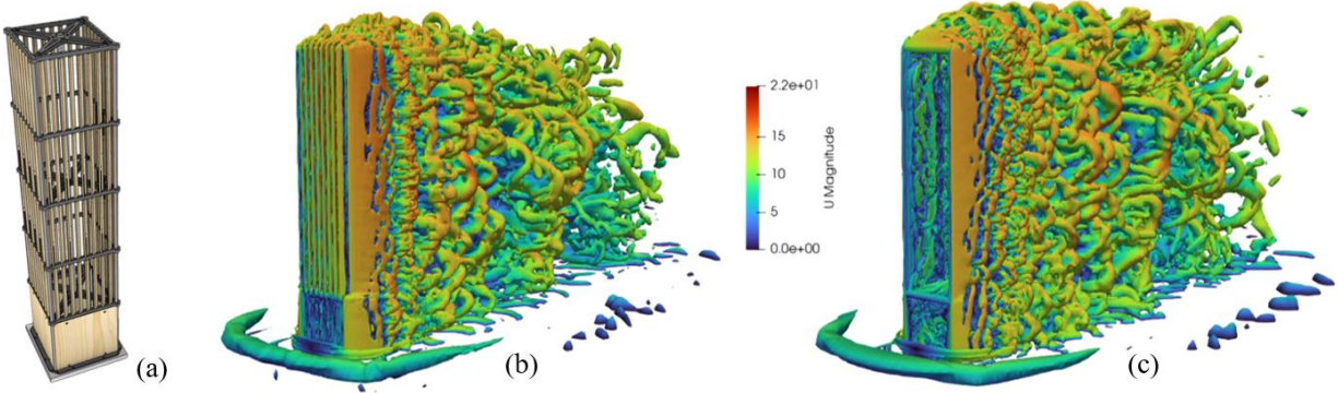
Figure 1: Overview of the considered porous prism: (a) geometry tested at Polytechnic of Milan, (b) LES with explicit model (Q-criterion) and (c) LES PVJ-based model.
